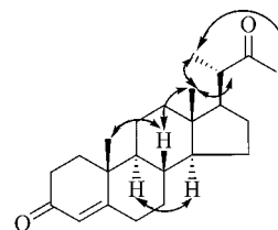
Figure 2. Selected NOEs in steroid 6
