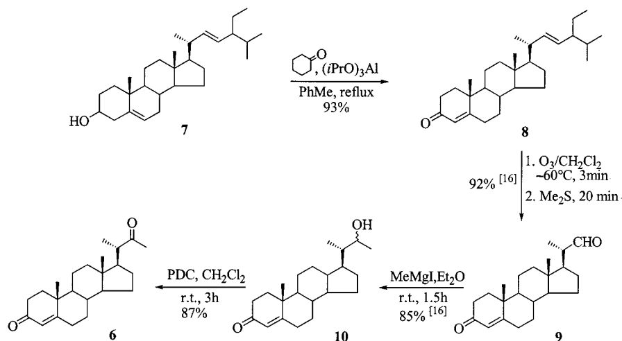
Scheme 1. Synthesis of steroid 6 from stigmasterol ( 7 )
